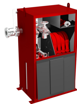
Hydrant with Foam Tank
