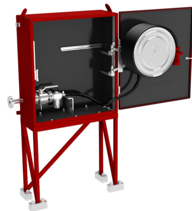
Hose Reel, Deck Mounted
